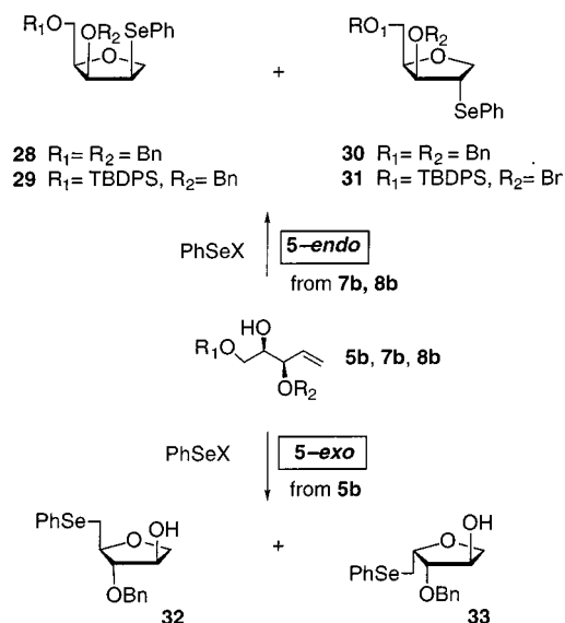
Scheme 8
